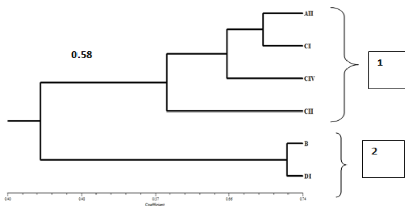
Fig. 6: UPMGA dendrogram showing the relationship among the isolates using the RAPD profile produced by the S gene primer, RAPD 1 primer and RAPD 2 primer. AII represents B. mycooides , B represents P. pneumotropica , CI represents B. polymyxa , CII represents P. aerogenes , CIV represents B. alvei , and DI represents S. aureus .
